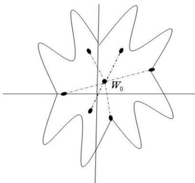
a starlike domain
