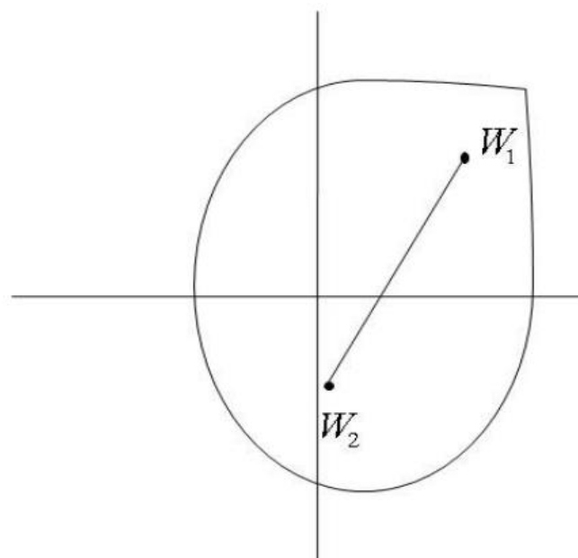
b convex domain
